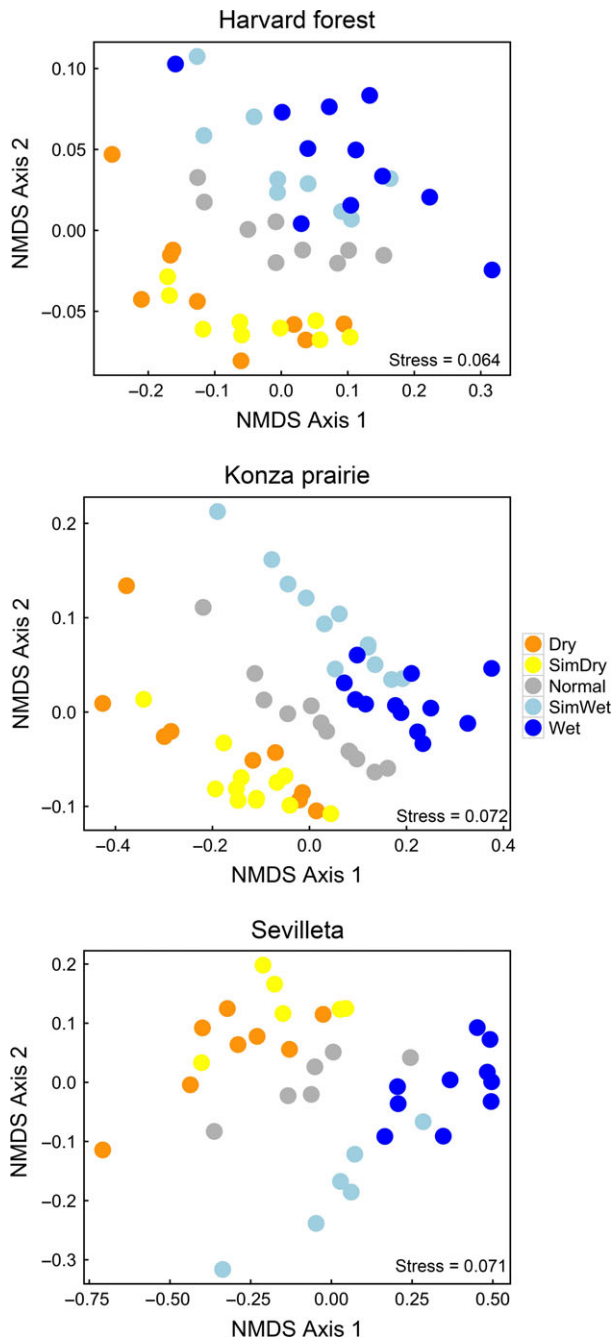
Fig. 3 Multidimensional scaling analysis of the impact of simulating extreme dry and wet years using ARMS (Gherardi & Sala, 2013) on five precipitation regime attributes: average precipitation event size, the number of precipitation events, the average length of dry periods between events (a dry day = <0.3 mm of precipitation), the number of extremely large (99th percentile) precipitation events, and the number of extremely long (95th percentile) periods of consecutive dry days (see Knapp et al. , 2015 for more detail). Simulations were performed in three ecosystem types selected to span a wide range of mean annual precipitation levels in the United States (NE Deciduous forest in Massachusetts, central mesic grassland in Kansas, and SW desert grassland in New Mexico). Dry years were simulated by removing a fixed proportion of each precipitation event by the amount necessary to reduce precipitation in normal years to a statistically extreme level. Extreme wet years were simulated by increasing by a constant proportion each precipitation event from normal years. Precipitation attributes from actual extreme dry, wet, and normal years are shown as well. PERMANOVA indicated that there were overall significant differences among groups ( P < 0.001 ) for all sites.
