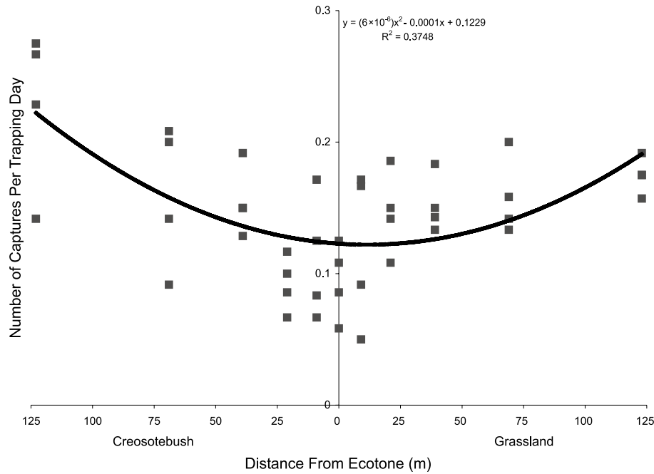
Fig. 4. Quadratic regression of total number of lizards captured with increasing distance from the ecotone. Lizard captures were standardized for differential trapping effort between years.
