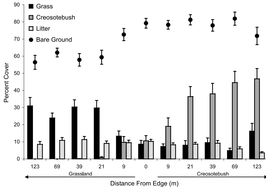
Fig. 2. Habitat characteristics with increasing distance from the ecotone. Measurements are percent coverage with the potential to have greater than 100%, owing to canopy coverage. All values are means \pm 1 SE.
