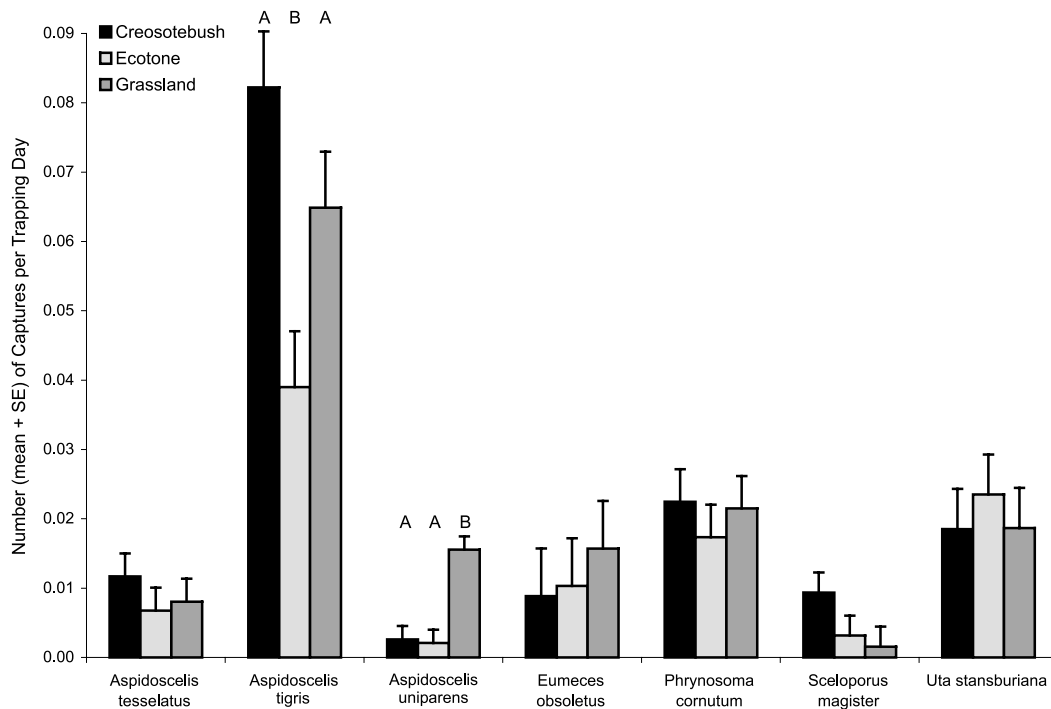
Fig. 5. Number of each lizard species captured in each habitat. Letters signify significant differences between habitats. All values are means \pm 1 SE.
