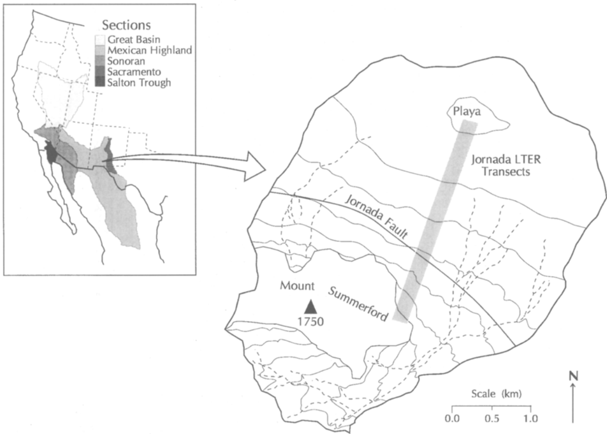
Fig. 1. Jornada LTER catchment showing location of the study transects, major drainage channels (dashed lines), and the location of the Jornada Fault. Contour interval is 15.5 m. Base elevation of the watershed is 1310 m at the center of the playa. Inset shows the extent of the five sections of the Basin and Range Physiographic Province in the western United States and northern Mexico (adapted from Peterson 1981 and Ordonez 1936), and the location of the Jornada LTER Site.
