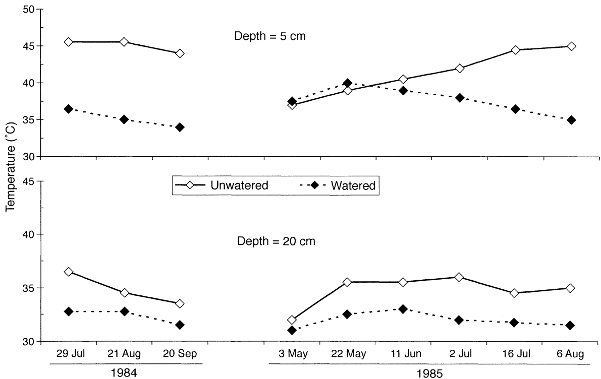
FIG. 3. Mean soil temperature ( ^{\circ}\text{C} , N = 4 ) at 5- and 20-cm depths on plots receiving only natural rainfall ("unwatered") and on plots receiving supplemental watering ("watered").
