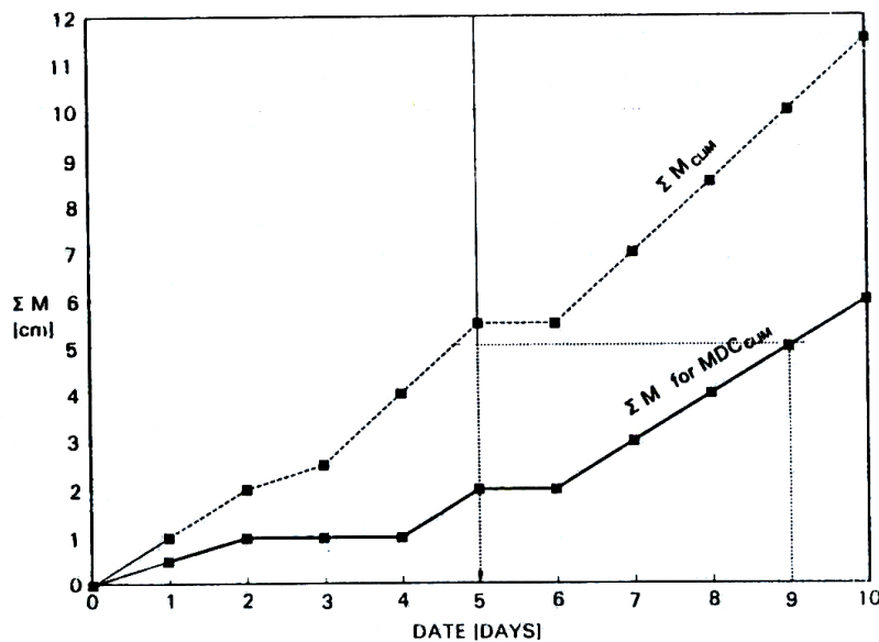
Fig. 2. Graphical determination of time shifting of snow covered area by a changed climate ( T + 1^{\circ}\text{C} ): In the present climate, a cumulative snowmelt depth of 5 cm is reached on day 9 (with new snow falls adjusted to T + 1^{\circ}\text{C} ), in the changed climate 5 cm is reached already on day 5.
