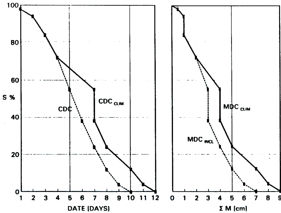
Fig. 4. Depletion curves of the snow coverage in the present climate (CDC) and in a changed climate (precipitation amounts doubled), CDC_{CLIM} , as derived from MDC_{CLIM} .
