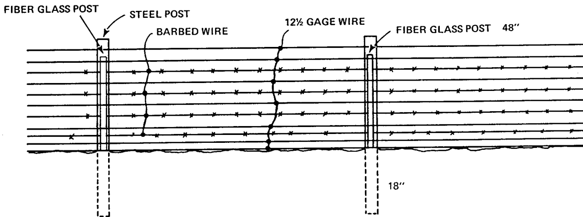
TYPICAL MODIFIED FENCE SECTION
