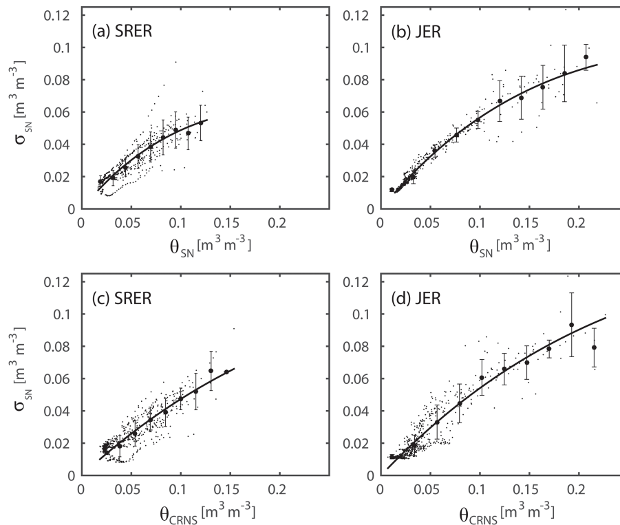
Figure 6. Soil moisture spatial variability as a function of the spatially averaged distributed sensor network ( \theta_{SN} , top) and the CRNS method ( \theta_{CRNS} , bottom) for (a, c) SRER and (b, d) JER. Bin averages and \pm 1 standard deviation are shown (circles and error bars) for bin widths of 0.015 \text{ m}^3 \text{ m}^{-3} at SRER and 0.025 \text{ m}^3 \text{ m}^{-3} at JER. Regressions for the relations of \sigma with \langle \theta \rangle are valid for the entire data set.
