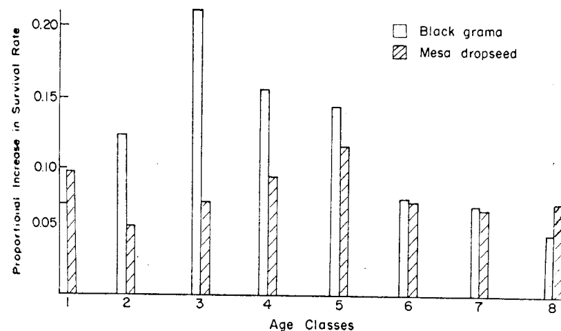
Fig. 2. The mean effect due to a change in effective moisture on the survival rates of black grama and mesa dropseed for given age classes.
