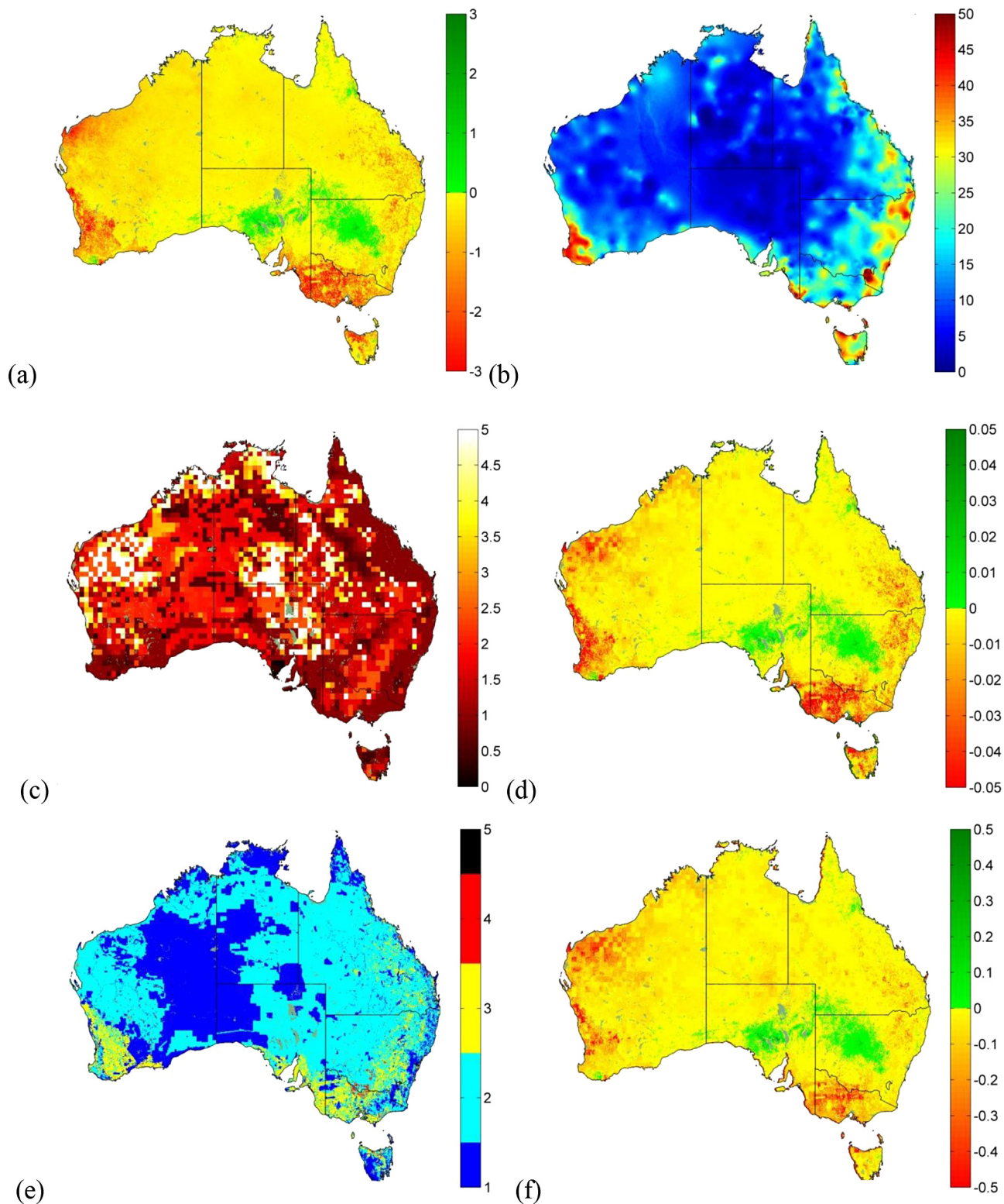
Figure 2. Maps for Australia showing (a) ^{137}\text{Cs} -derived median net (1950s–1990) soil redistribution ( \text{t soil ha}^{-1} \text{yr}^{-1} ). Positive values represent sites of net gain, while negative values are those of net loss. (b) Soil organic carbon (SOC) stocks ( \text{tC ha}^{-1} ; 0–10 cm). (c) Enrichment ratio at 50 km resolution. (d) SOC net redistribution ( \text{tC ha}^{-1} \text{yr}^{-1} ). (e) Land use (see Table 1). (f) SOC net redistribution as a proportion ( \% \text{yr}^{-1} ) of SOC stocks.
