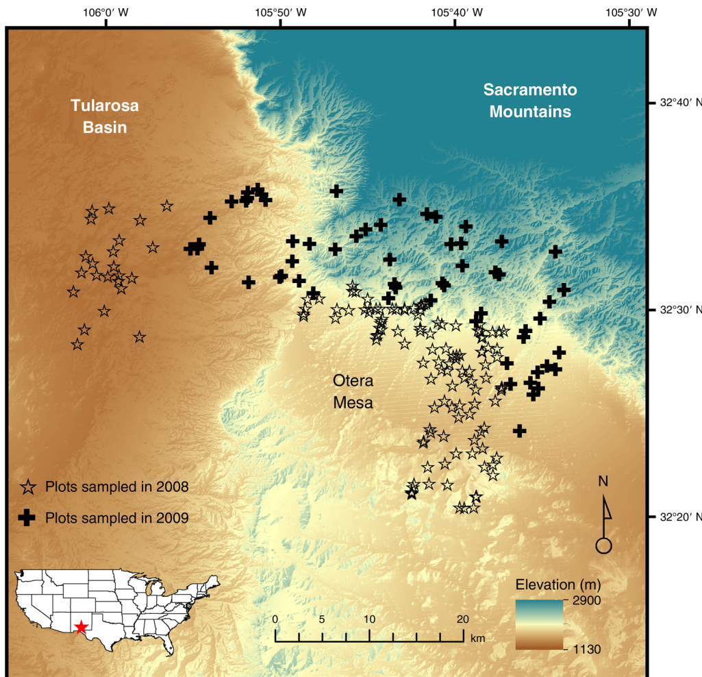
FIG. 2. Study area map showing the location of plots sampled in 2008 and 2009 in southern New Mexico, USA. Plots were located across five ecological sites on Otera Mesa and the eastern fringe of the Tularosa Basin.
