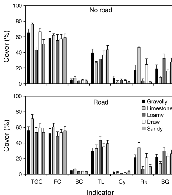
Fig. 3. Summary of ground cover characteristics (2008 and 2009 combined) for the five ecological sites. Data were collected along transects using the line–point intercept (LPI) method (see Methods section). Ground cover characteristics include: total ground cover (TGC, including foliar and basal cover, litter, cyanobacteria and rock cover), foliar cover (FC, of plant canopies), plant basal cover (BC), total litter cover (TL), cyanobacteria crust cover (Cy), rock cover (Rk), and bare ground cover (BG, including that beneath overhanging plant canopies).
