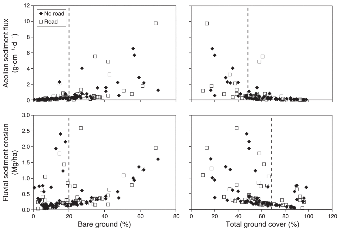
FIG. 5. Graphs showing the relationship between simulated aeolian horizontal sediment flux (top), soil loss due to fluvial sediment erosion (bottom), and the fractional cover of bare ground and total ground cover. Data are shown from all ecological sites, at plots without and with adjacent roadways in 2008 and 2009. Dashed lines indicate proposed thresholds for horizontal sediment flux and soil erosion.
