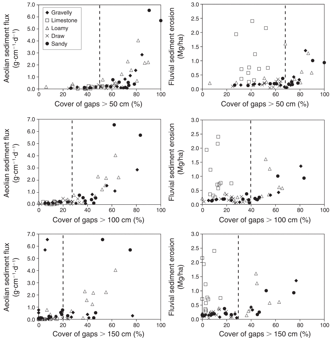
FIG. 6. Selected graphs showing the relationship between simulated aeolian horizontal sediment flux, soil loss due to fluvial sediment erosion, and the percent cover of canopy gaps larger than 50 cm, 100 cm, and 150 cm. Data are shown for all five ecological sites, at plots without adjacent roadways sampled in 2008 and 2009. Dashed lines indicate proposed thresholds for horizontal sediment flux and soil erosion.
