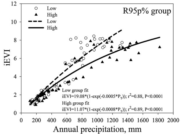
Figure 4. Relation of production across precipitation gradients for 11 sites for two groups (Low: R95p% < 20\% ; High: R95p% \geq 20\% ). See Table 2 for R95p% definitions. The relations were significantly different for the two groups ( F_{2,106} = 18.51 ; P < 0.0001 ).
