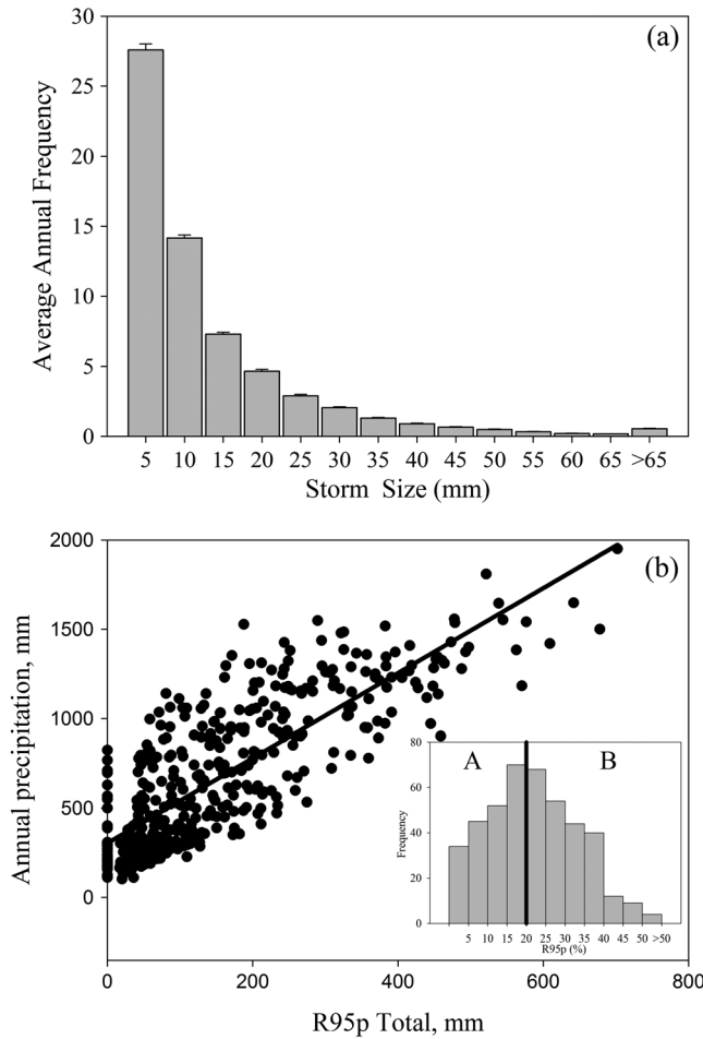
Figure 2. (a) Frequency analysis of size of precipitation events for the whole site year data set. (b) The contribution of extreme rainfall events to total precipitation for the whole data set. The regression coefficient of correlation ( r^2 ) is 0.66 ( P < 0.01 ), as stated in Table 3. The inset shows the frequency of R95p%. The thick solid line within the inset indicates the threshold to define the two groups based on R95p% of all site year data.
