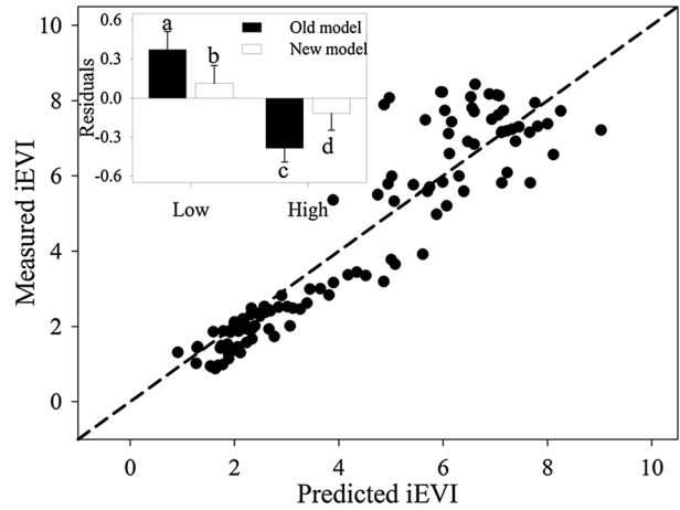
Figure 6. Comparison between predicted and measured iEVI with the new model [Equation (3)] across all sites. The inset shows the comparisons of the mean residual for Low and High groups (Figure 1b) with the old [Equation (2)] and new [Equation (3)] models. Different letters indicate significant differences at P < 0.05 .
