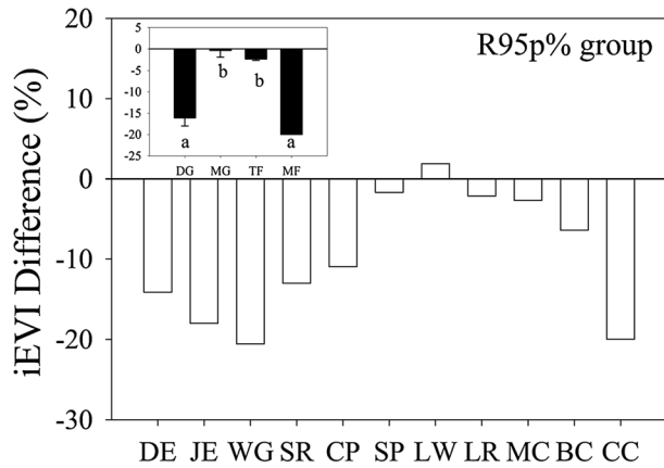
Figure 3. Comparison of iEVI relative difference of years with similar annual precipitation but different R95p% group (years in the Low and High groups; iEVI difference = (iEVI_{High} - iEVI_{Low}) / iEVI_{Low} \times 100 across 11 sites. For each site, the years with similar annual precipitation were selected to compare the iEVI differences in the two groups. The inset shows the average iEVI difference combined into biome types. Different letters indicate significant differences at P < 0.05 .
