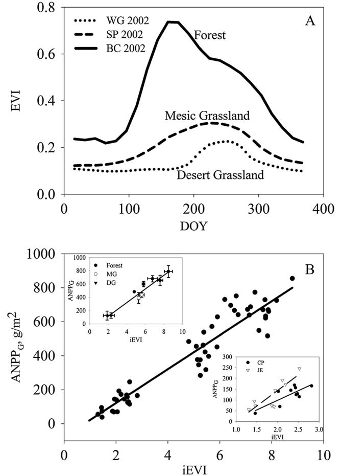
Figure 1. (a) An example of 1-year smoothed EVI time series for desert grassland (DG), mesic grassland (MG), and forest. (b) Relationship between annual ANPP G and the corresponding iEVI derived from MODIS data during the 2000–2009 period for nine selected sites across biomes. The solid line shows the linear regression ( R^2=0.90 ; P<0.0001 ; RMSE=82.60). The top inset shows the site average of ANPP G and iEVI (regression model, R^2=0.94 ; P<0.0001 ; RMSE=65.87). Error bars are the standard deviations. The bottom inset shows the relationships at sites CP and JE ( R^2=0.50 and 0.74 ; RMSE=29.29 and 36.89, respectively; P<0.01 ).
