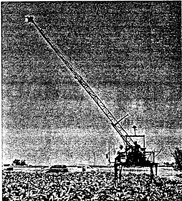
Figure 4. A boom-type data acquisition system mounted on a high-clearance tractor at the ARS Water Management Research Center in Ft. Collins, Colorado.
