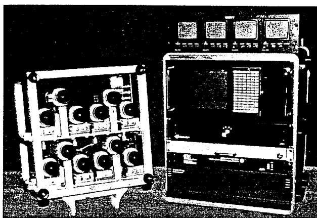
Figure 2. The airborne digital video imaging systems (ADVIS) developed at Weslaco, Texas.
