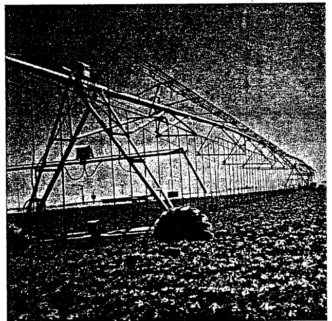
Figure 5. The linear move system serving as a platform for the Agricultural Irrigation Imaging System, AgIIS Ag Eyes, in Phoenix, Arizona.
