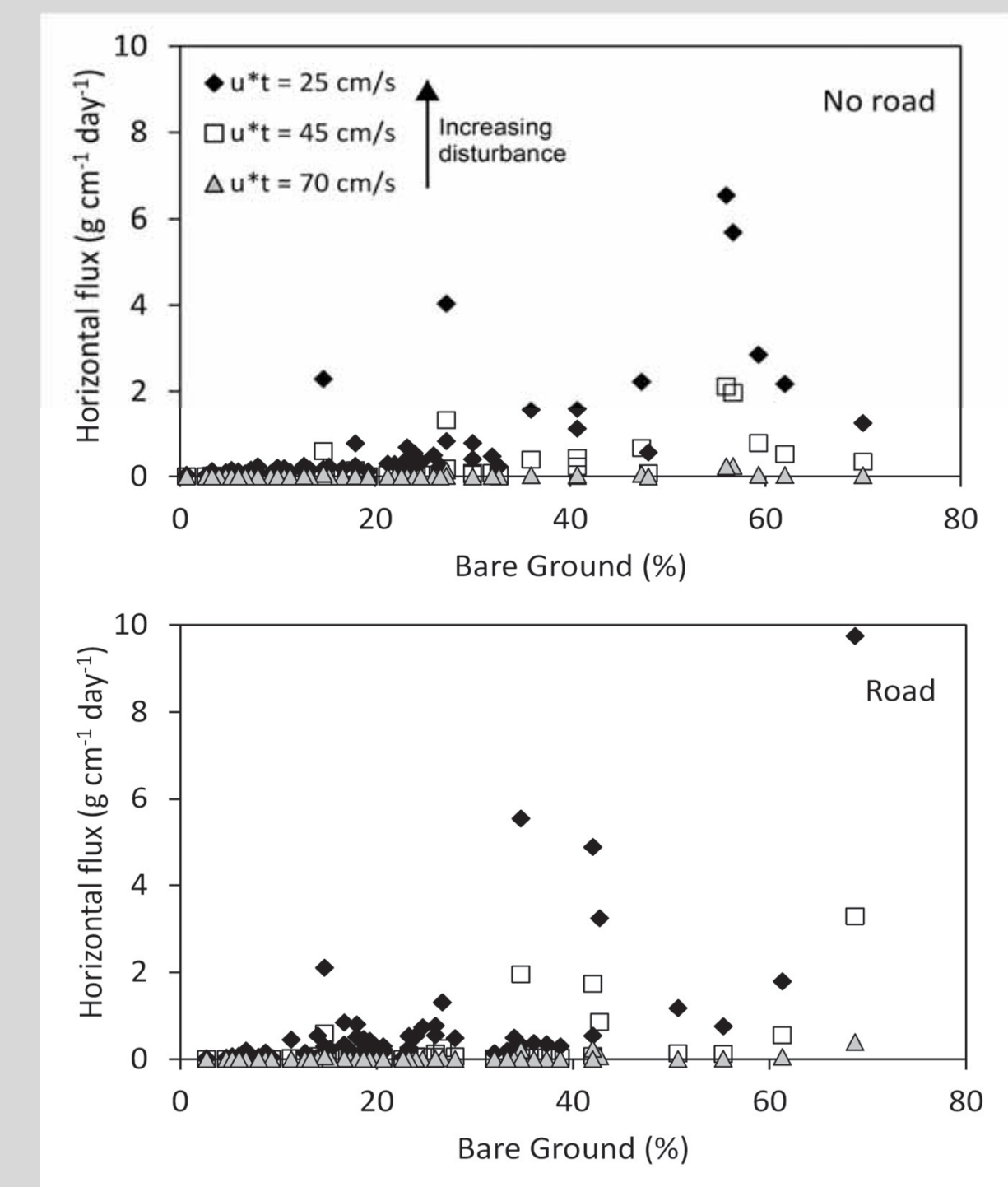
Fig. 8: Modelled effect of soil disturbance on the sediment flux due to wind erosion, represented by a change in the soil entrainment threshold ( u_{*t} ).
