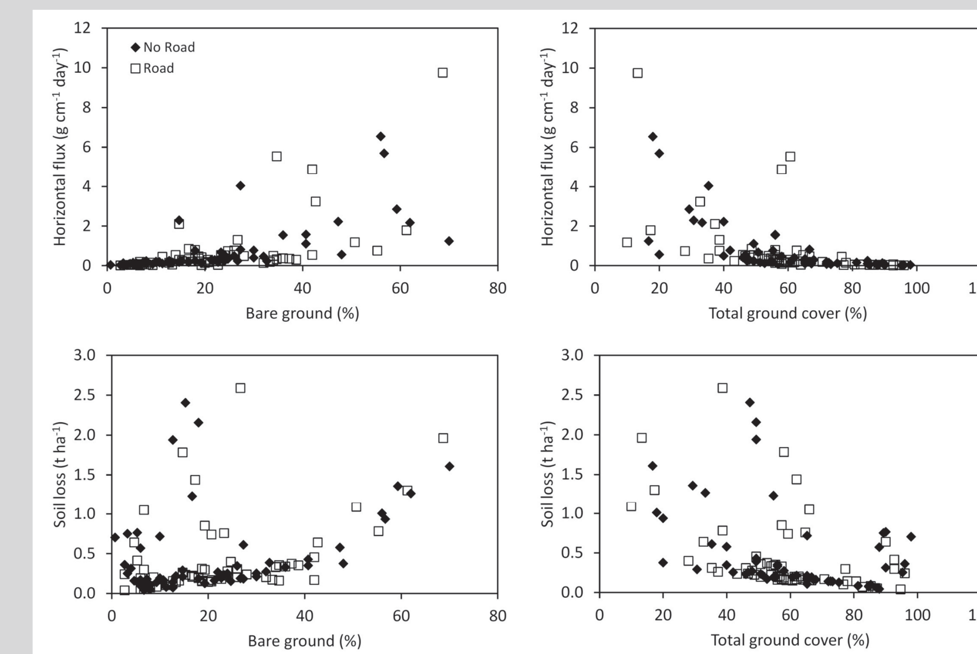
Fig. 6: The relationship between simulated horizontal sediment flux due to wind erosion, soil loss due to water erosion and the measured fractional cover of bare ground and total ground cover for the 120 study plots.
