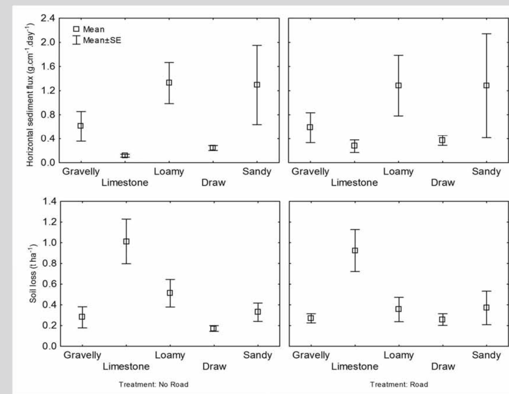
Fig. 3: Simulated wind and water erosion rates for the five ecological sites, separated for those away from and adjacent to road disturbances.
