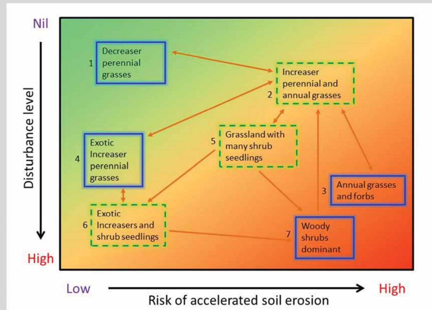
Fig. 1: Generalised state-and-transition model 1 showing potential interactions between disturbance levels, ecological state changes and accelerated soil erosion.
